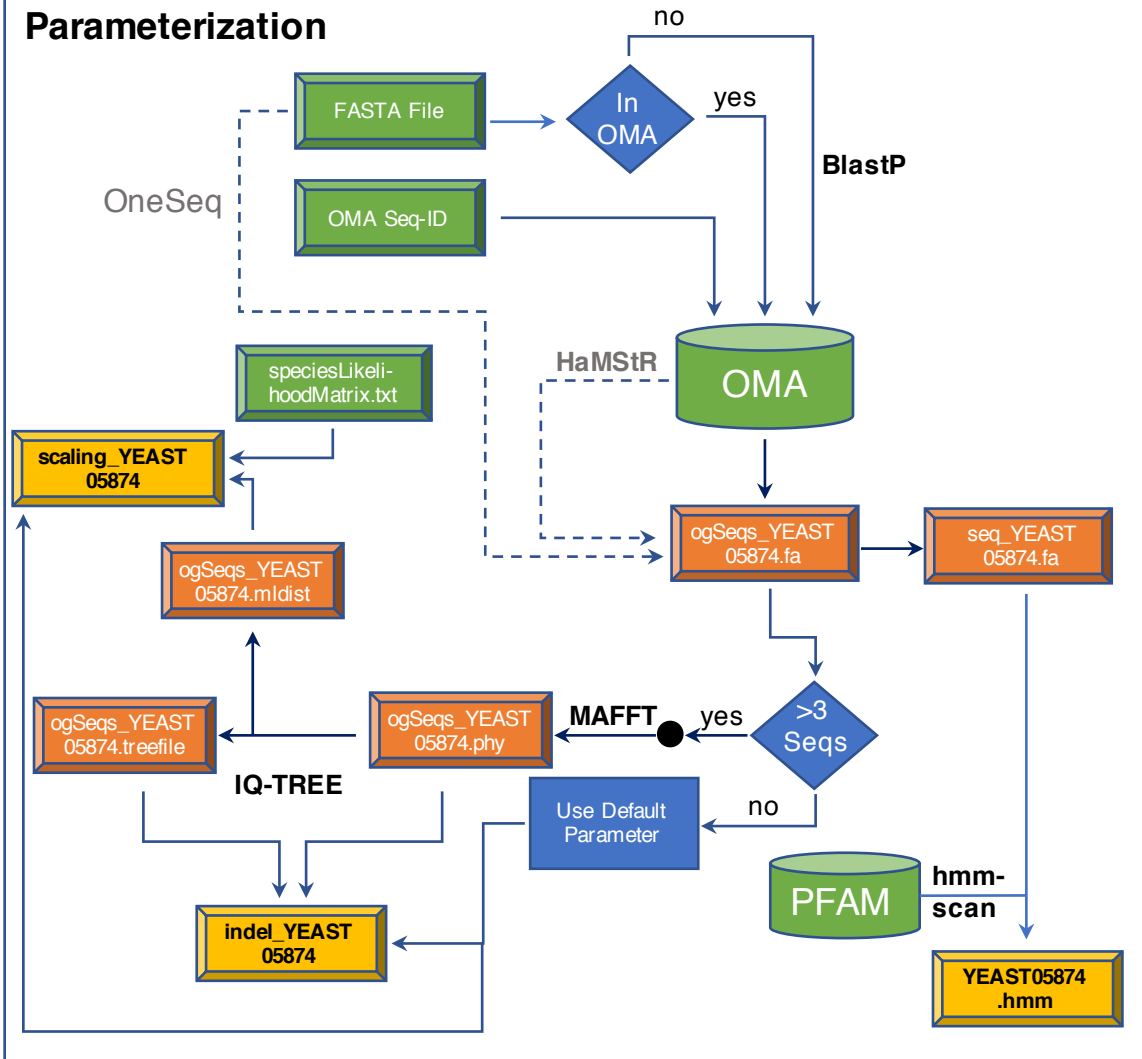
protTrace Workflow – Workflow of the protTrace analysis distinguished into the categories Parameterization, Traceability calculation, and visualization. Boxes in green denote input files, boxes in orange represent meta-information, which is generated in the course of the analysis, and yellow boxes indicate output files that are generated as a result of an analysis. Arrows represent individual analysis steps, where the arrow style indicates whether the analysis step is obligatory (solid), or optional (dashed). Analysis steps that require the calling of external programs are indicated by the program name next to the corresponding arrow. Obligatory dependencies on 3d party software are represented by bold face black program names, those that are optional are indicated by grey font color.
